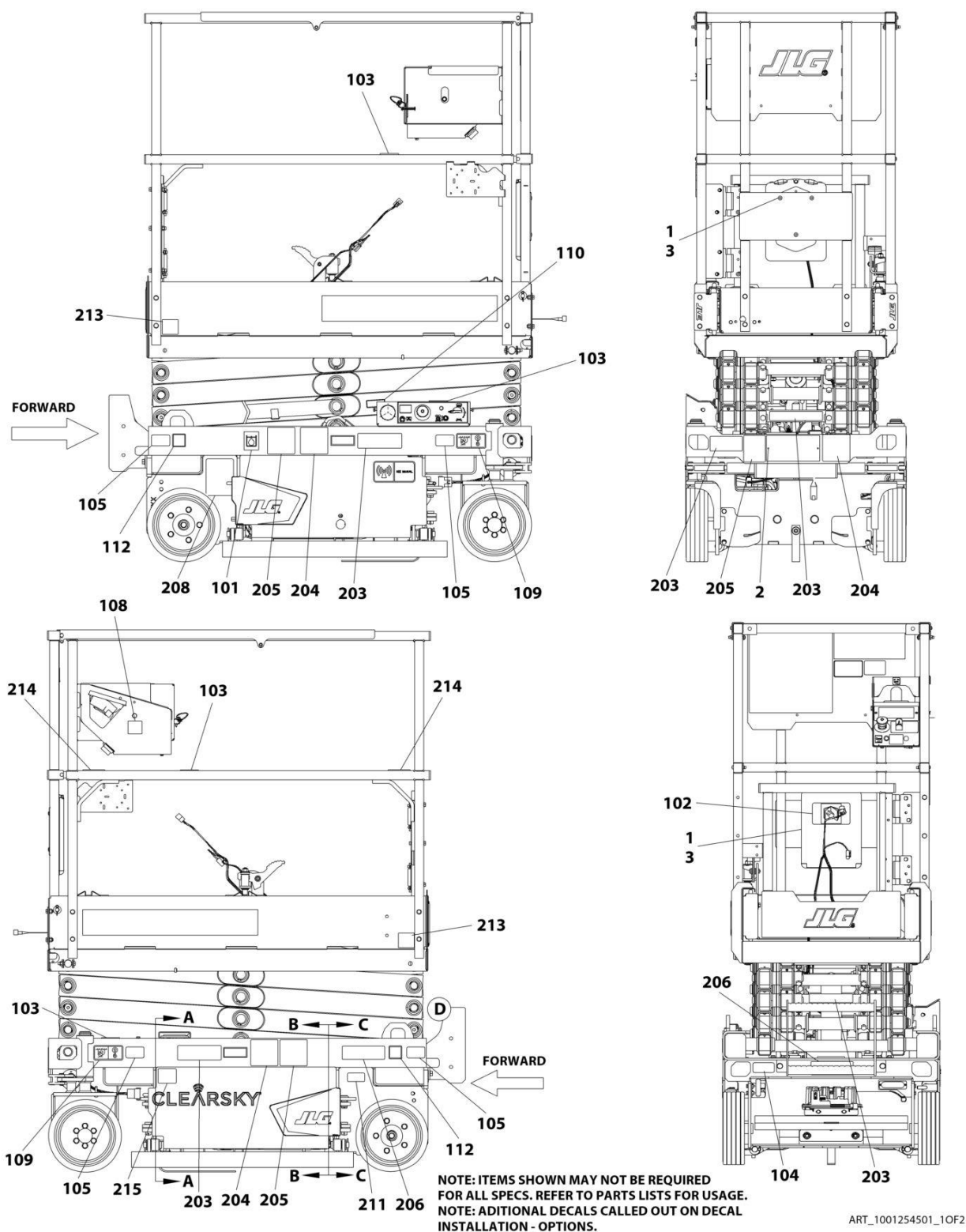
FIGURE 8-5. DECAL INSTALLATION (CSA SPECS)
