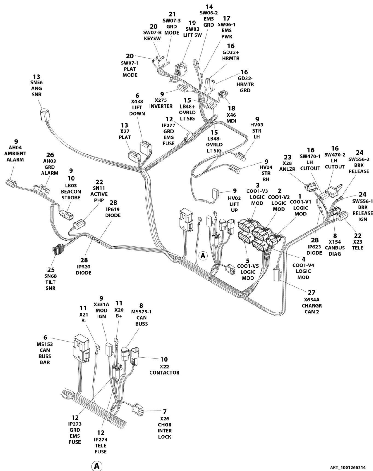
FIGURE 7-23. CHASSIS HARNESS (WITH PLATFORM DRIVE SELECT SWITCH) (CHINA & MEXICO BUILT MACHINES)
