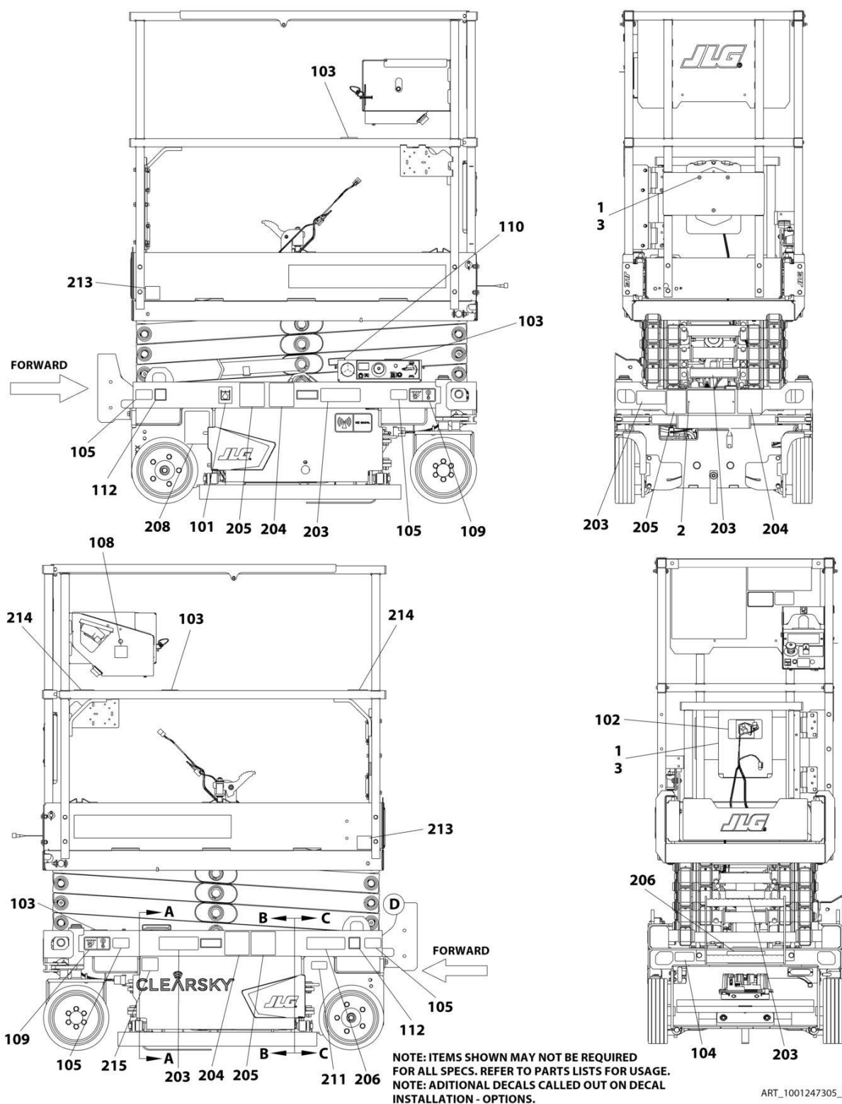
FIGURE 8-3. DECAL INSTALLATION (CE SPECS)
