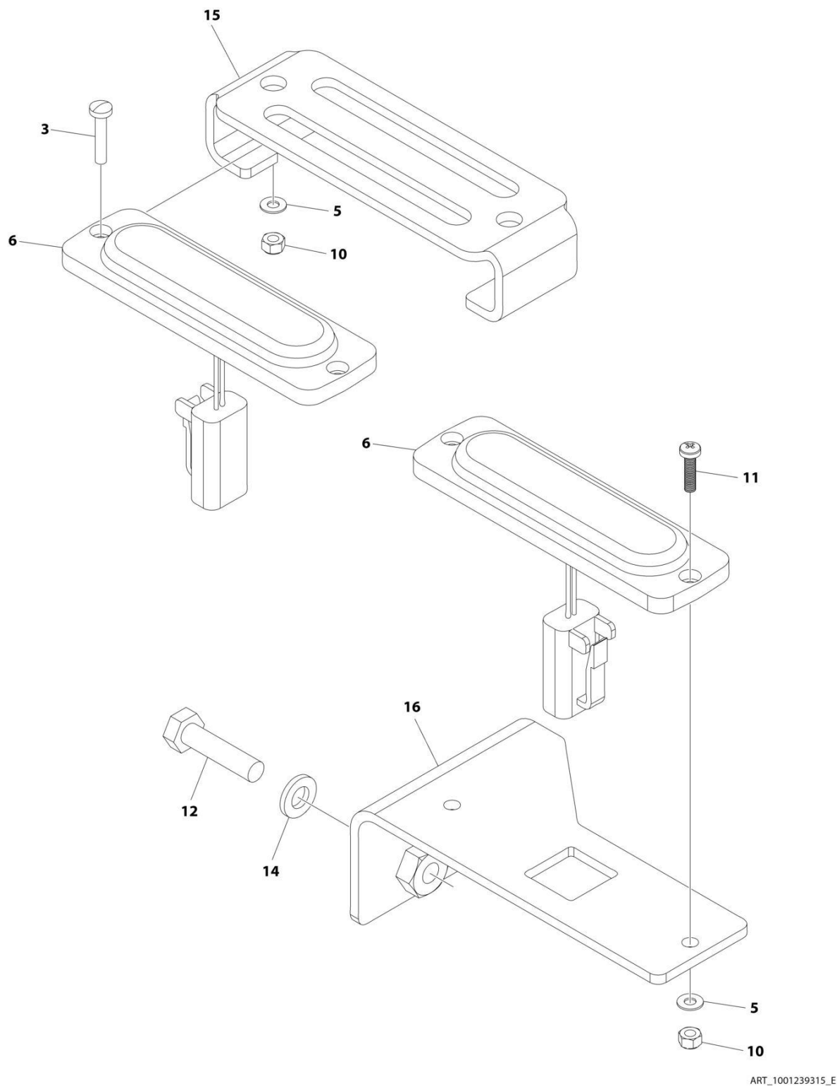
FIGURE 1-24. STROBE LIGHT INSTALLATION - DUAL (AMBER) (WITH GUARD) (SN B200062116 through B200065277)
