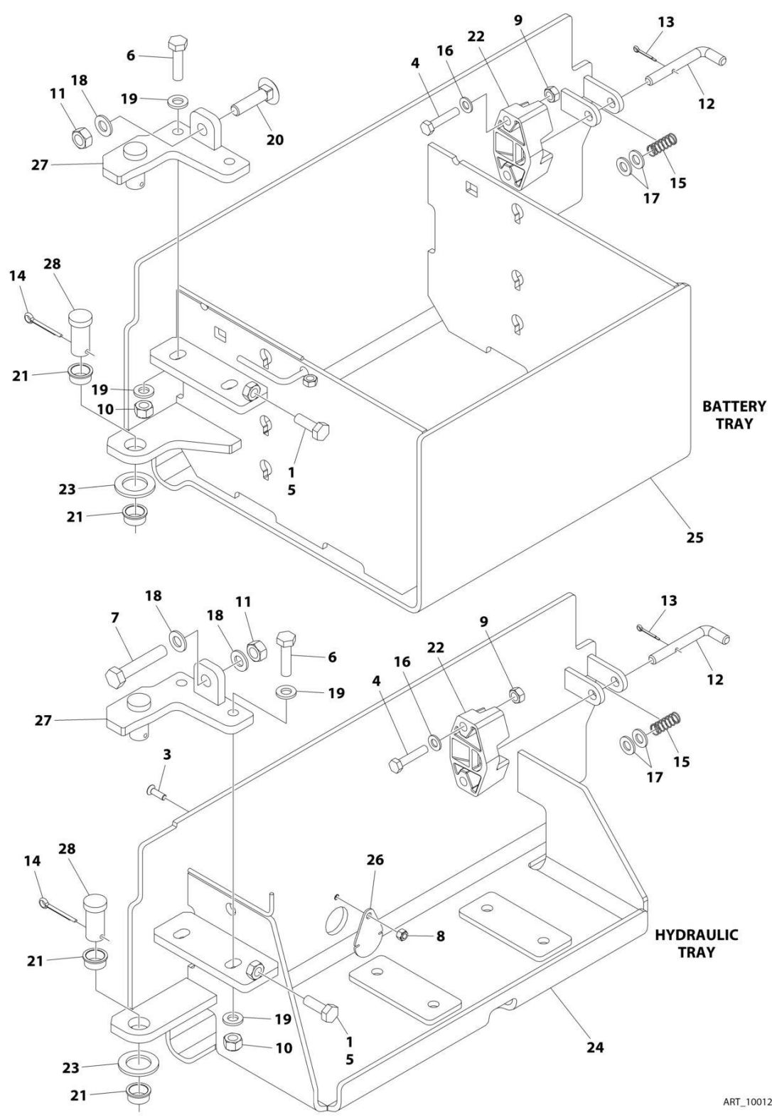
FIGURE 2-13. DOORS INSTALLATION
